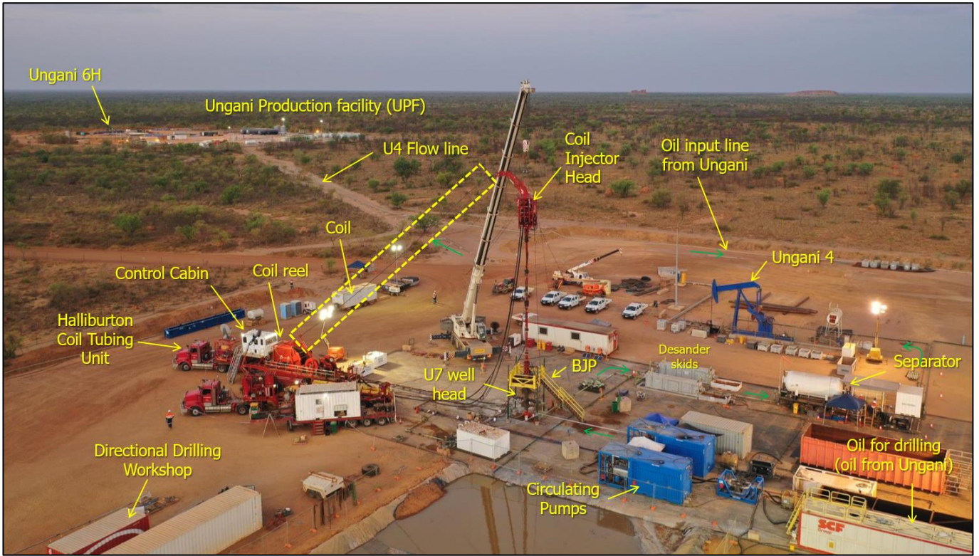
Coil drilling spread on Ungani 7H
